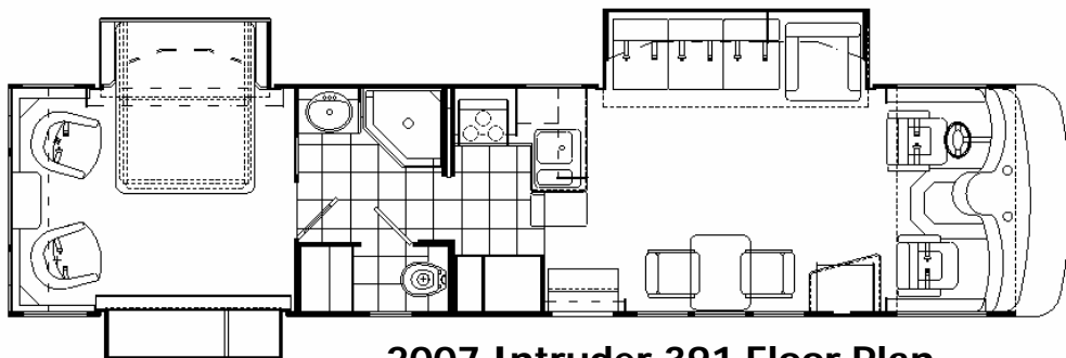
2007 Intruder 391 Floor Plan
