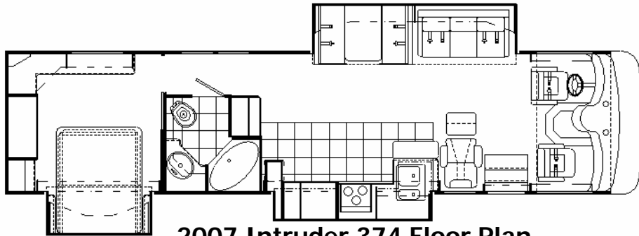
2007 Intruder 374 Floor Plan
